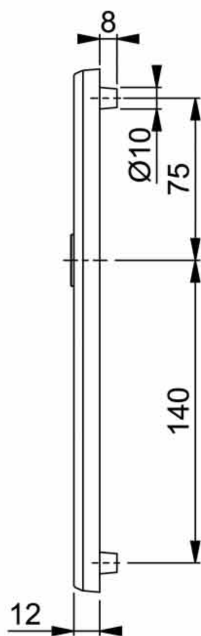
Type B Backplate 92/215 Centres
